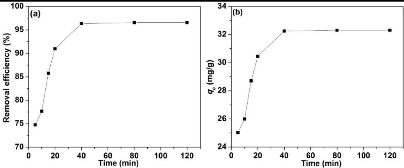
Fig. 6: Relationship of contact time with respect to Cu 2+ concentration of 100 mg L -1 at 25°C, 150 rpm, adsorbent concentration 3 g L -1 (a) removal efficiency and (b) adsorption capacity.
