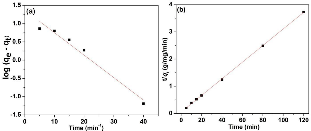
Fig.7: Kinetic model graphs on Cu 2+ uptake adsorption by AC1: (a) Lagergren 1 st order and (b) 2 nd order model correspondingly.
